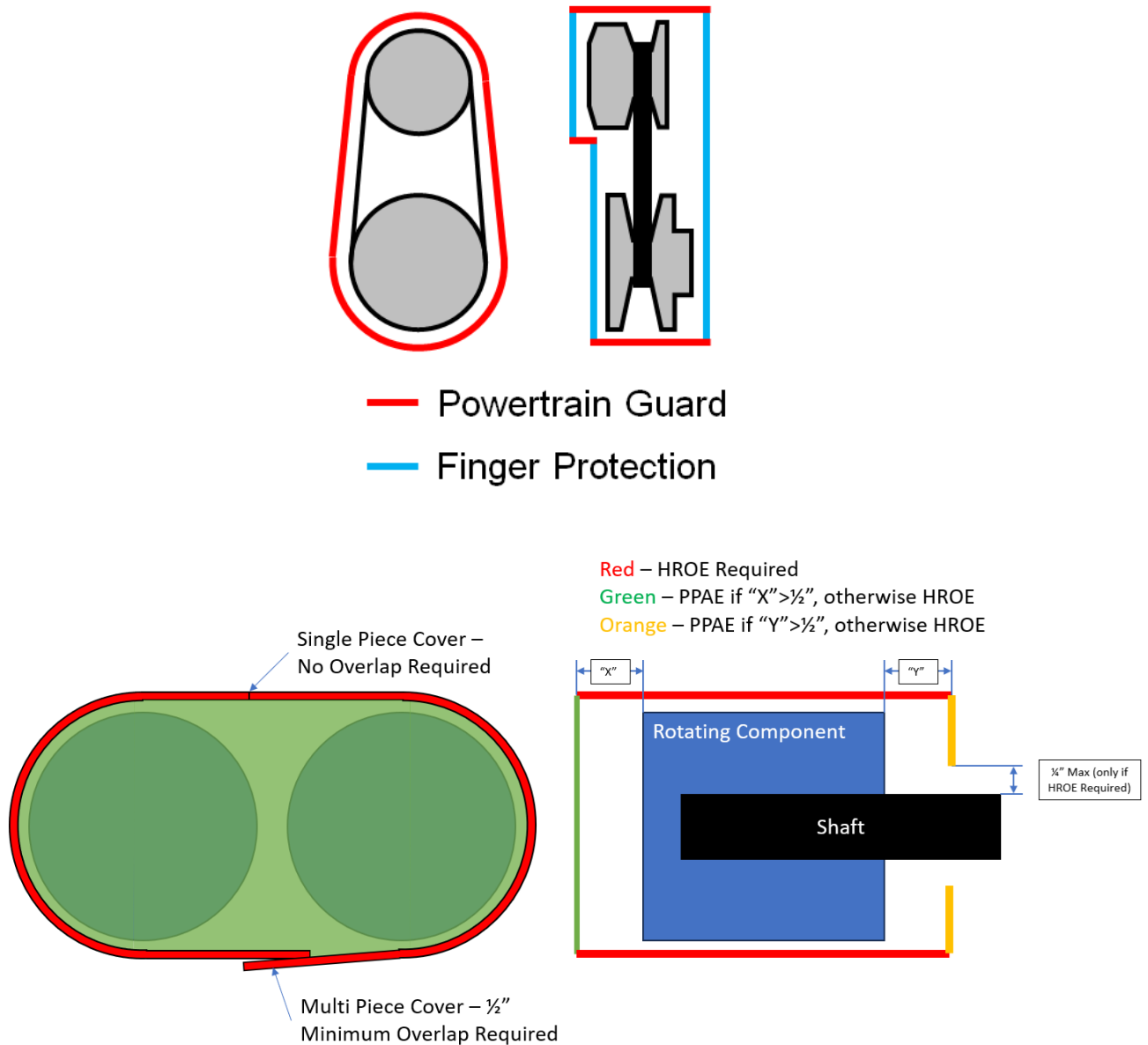
Figure B-54: Powertrain Guard Extent example on a CVT
