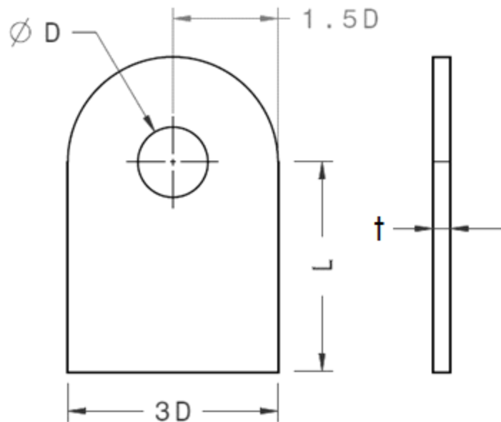
Figure B-58: Required Tab Drawing
